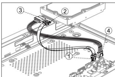
Figure 2-10 Connect Cables
