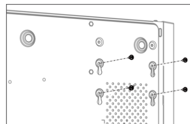
Figure 2-11 Fix HDD to Device Bottom
