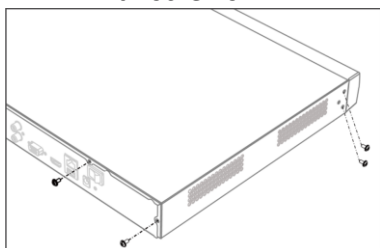
Figure 2-9 Remove Cover
